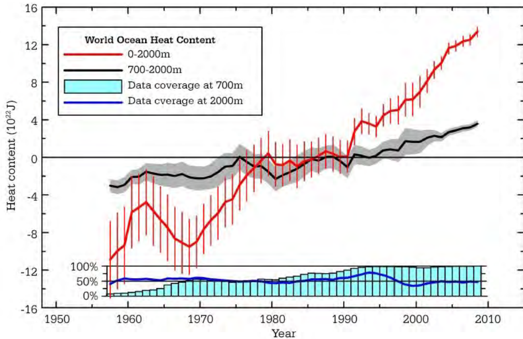
Figure 14: Time series of global ocean heat content demonstrating an increase in heat content (measured as 10^{22} J) for both the 0-2,000 m and 700-2,000 m layers of the ocean since 1955. The red line demonstrates the 0-2,000 m layer and the black line demonstrates the 700-2000 m layer. Measurements are based on running averages over five-year periods, relative to 1955-2006. The vertical red bars represent \pm 2 times the standard error of the mean 0-2,000 m estimates and the grey-shaded area represents \pm 2 times the standard error about the 700-2,000 m estimates. The blue bar chart at the bottom represents the percentage of one-degree squares (globally) that have at least four 5-year one-degree square anomaly values used in their computation at 700 m depth. Blue line is the same as for the bar chart but for 2,000 m depth.
