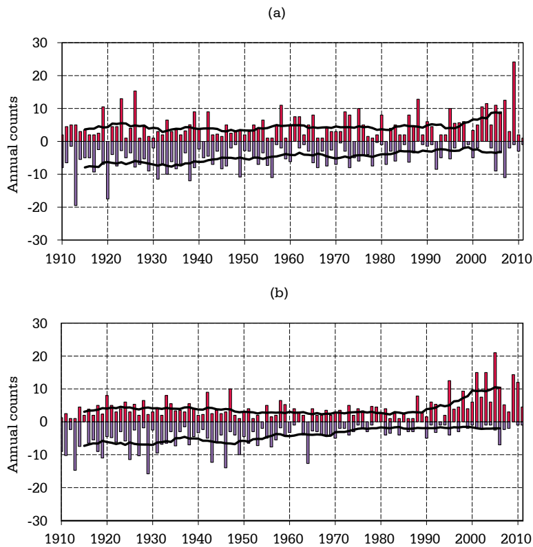
Figure 34: Number of record high temperatures (red bars) and record low temperatures (purple bars) per year for (a) daily maximum temperature, and (b) daily minimum temperature at Australian climate reference stations for the period 1910-2011.
