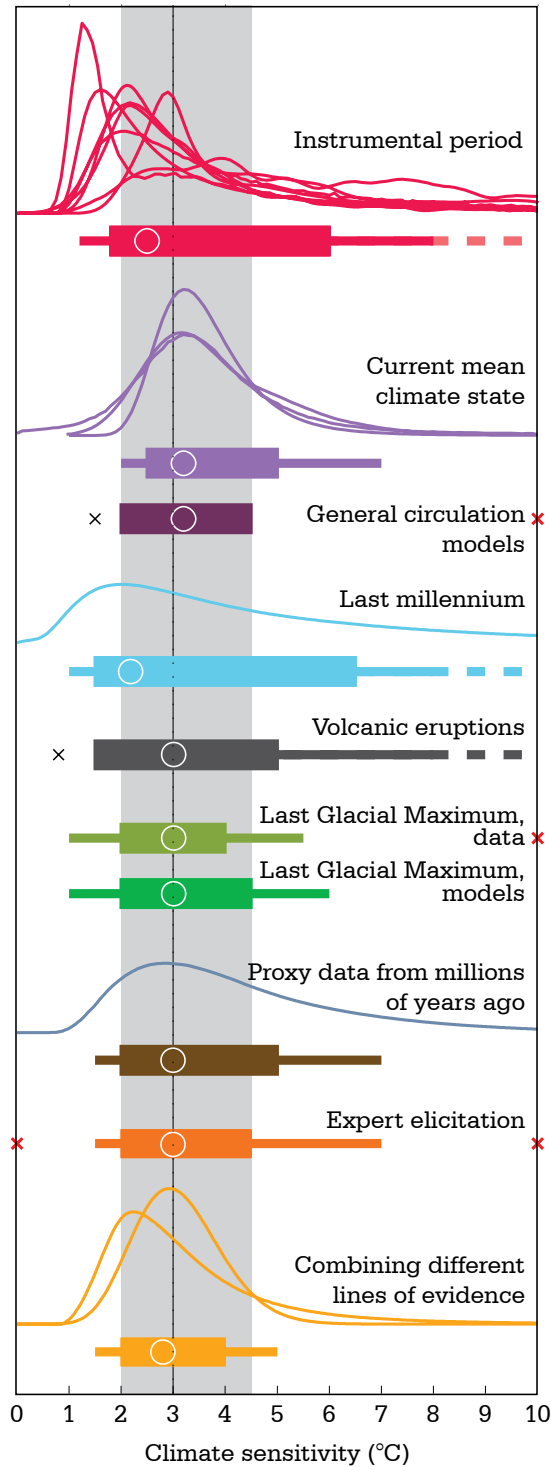
Figure 30: Distribution and ranges for climate sensitivity from different lines of evidence. The most likely values (circles), likely (bars, more than 66% probability) and very likely (lines, more than 90% probability) ranges are subjective estimates by the authors based on the available distributions and uncertainty estimates from individual studies, taking into account the model structure, observations and statistical methods used. Values are typically uncertain by 0.5°C. Dashed lines indicate no robust constraint on an upper bound. Distributions are truncated in the range 0-10°C; most studies use uniform priors in climate sensitivity. Single extreme estimates or outliers (some not credible) are marked with crosses. The IPCC (2007) likely range and most likely value are indicated by the vertical grey bar and black line, respectively.
